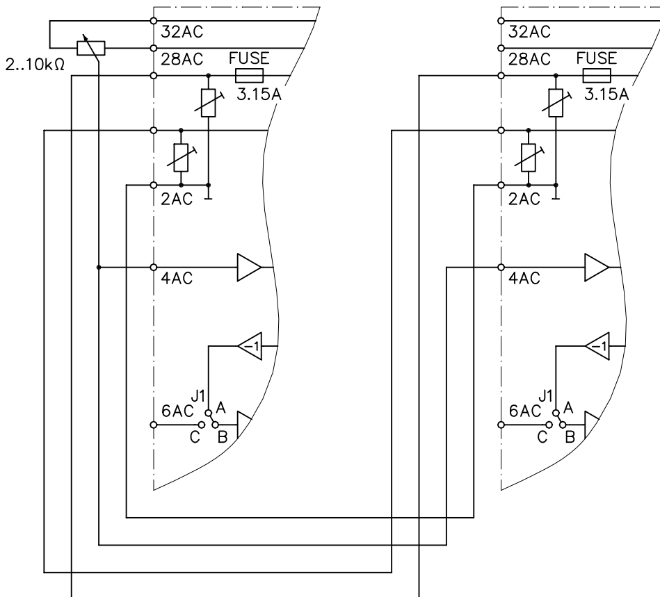
Controllo di due HCV in parallelo (con 2 schede VPD/AD) Two HCV in parallel operation (with two VPD/AD cards)
