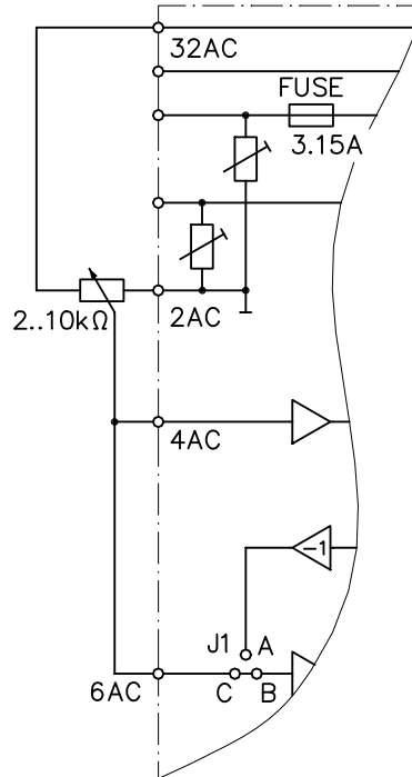
Controllo di due HCV in parallelo (con 2 schede VPD/AD) Two HCV in parallel operation (with two VPD/AD cards)
