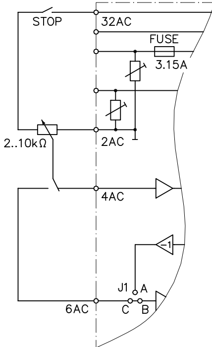
Controllo di due HCV in parallelo (con 2 schede VPD/AD) Two HCV in parallel operation (with two VPD/AD cards)
